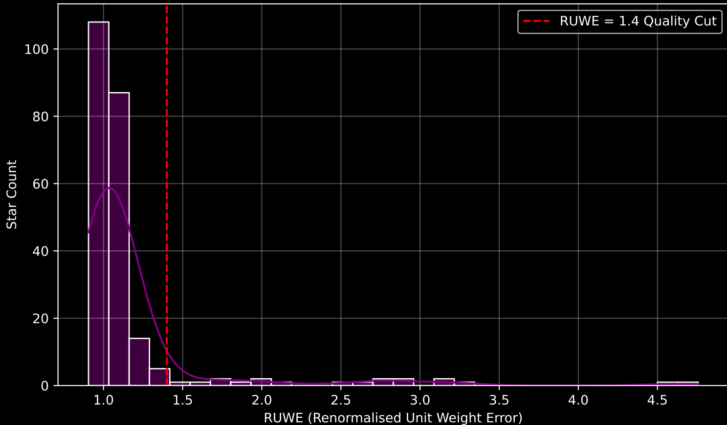
GALAH DR4 Field [1143] RUWE Distribution (n= 233)
