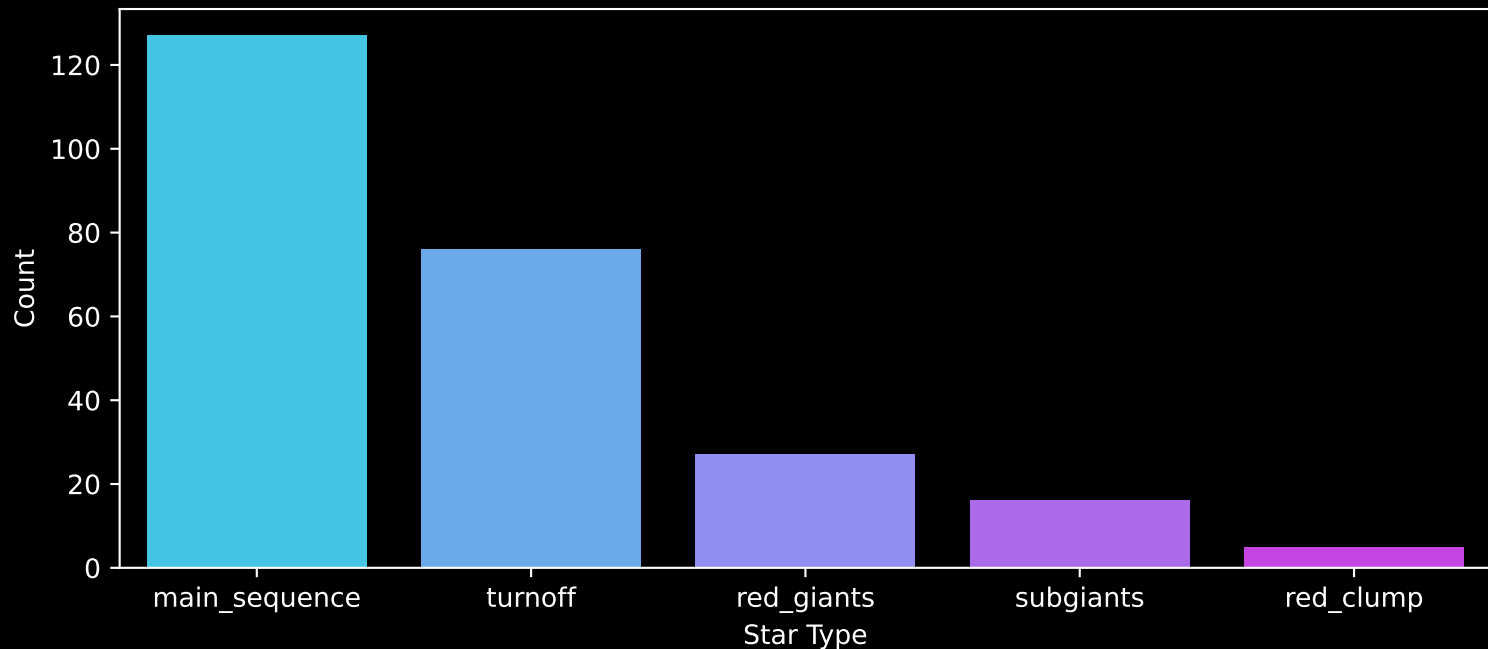
GALAH DR4 Field: [1143] Count plot of Star Type
